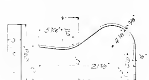
Figs. 4903-4. BRAKE-BEAM RELEASE-SPRING.
